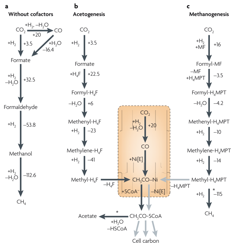
Figure 3 | Chemical and biochemical reactions. A schematic of the H 2 -dependent conversions of CO 2 to CH 4 without cofactors ( a ) and with cofactors ( b,c ) in acetogens (to acetate) and methanogens growing on H 2 and CO 2 . The numbers next to the arrows indicate the approximate change in free energy ( \Delta G^\circ ) at 25°C and pH 7 ( \Delta G^\circ ) in kJ per mole. The thermodynamic values are taken from REFS 55,56. For details of the biologically catalysed reactions, see the review by Maden 55 . For details of the reactions without cofactors under hydrothermal conditions, in which the thermodynamic values provided do not directly apply, see REF. 101. The dotted oval represents bifunctional CO dehydrogenase/ acetyl-coenzyme A (acetyl CoA) synthase (CODH/ACS), a conserved enzyme that is common to the acetyl-CoA pathway of CO 2 reduction in both acetogens and methanogens. The enzymes that are involved in methyl synthesis in acetogens and methanogens are not evolutionary related, even though similar chemical steps are involved 55,63 . This has been interpreted to mean that the overall exergonic chemical conversions are more ancient than the enzymes that catalyse them in modern cells. Although all reactions shown are reversible, arrows are shown in only one direction for simplicity. The asterisks at the methyl-H 4 MPT to CH 4 conversion and the acetyl-CoA to acetate conversion 54 indicate that several enzymes and cofactors that are not shown here are involved 55 . In both acetogens 54 and methanogens 53 , net energy conservation (ATP gain) involves the generation of ion gradients using the overall reaction shown. This chemiosmotic potential is then harnessed by an ATPase. The coupling site in methanogenesis (not shown) entails the conversion of methyl-H 4 MPT to CH 4 (REF. 53); the coupling site in acetogenesis (not shown) has recently been suggested to involve a ferredoxin-NAD + oxidoreductase 102 . The formate to formyl-H 4 F conversion in acetogens involves ATP hydrolysis (not shown), which lowers \Delta G^\circ for the reaction to -10 kJ per mole 55 ; the chemiosmotic potential is required for the synthesis of formyl-MF in methanogens 53 . For both acetogens and methanogens, black arrows indicate reactions that are involved in core ATP synthesis, whereas grey arrows indicate that a portion of the total carbon flux is used to satisfy the carbon needs of the cell. H 4 F, tetrahydrofolate; H 4 MPT, tetrahydromethanopterin; HSCoA, coenzyme A; MF, methanofuran; Ni[E], an Fe-Ni-S cluster in CODH/ACS. Part a adapted, with permission, from REF. 101 © (2006) National Academy of Sciences. Parts b,c adapted, with permission, from REF. 55 © (2000) Portland Press.
